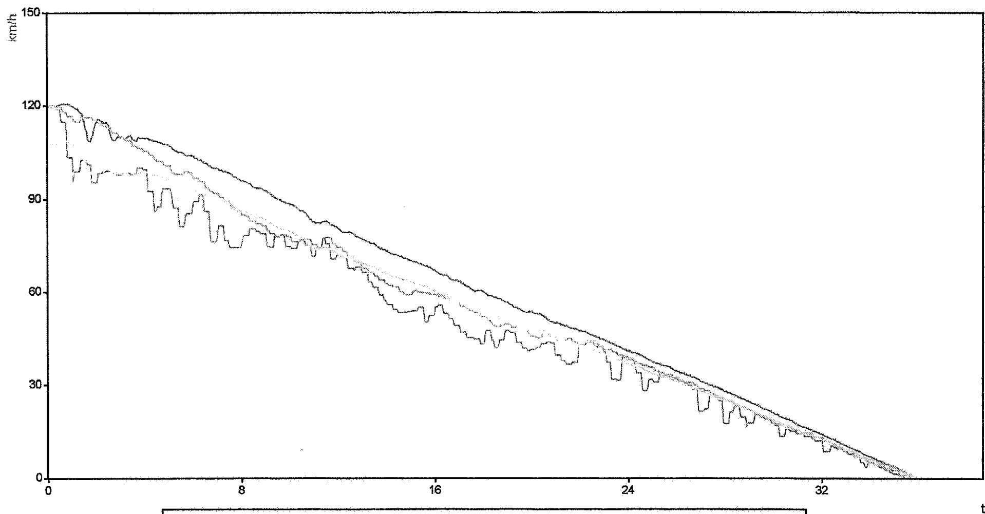
Slide evaluation 01apr18 (Safety purely pneumatic no MTB) - M1axle 4 - GM > 35% train speed SpeedRefM1 M1_WSP4 90% of train speed
