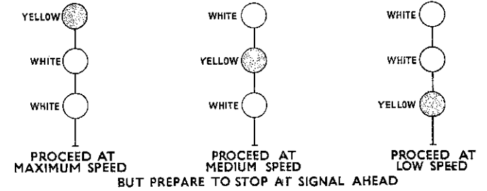
Fig. 2 Caution indications
