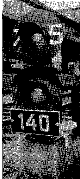
Two-unit signal at ground level, for medium (45 m.p.h.) and low (28 m.p.h.) speed, in station area
