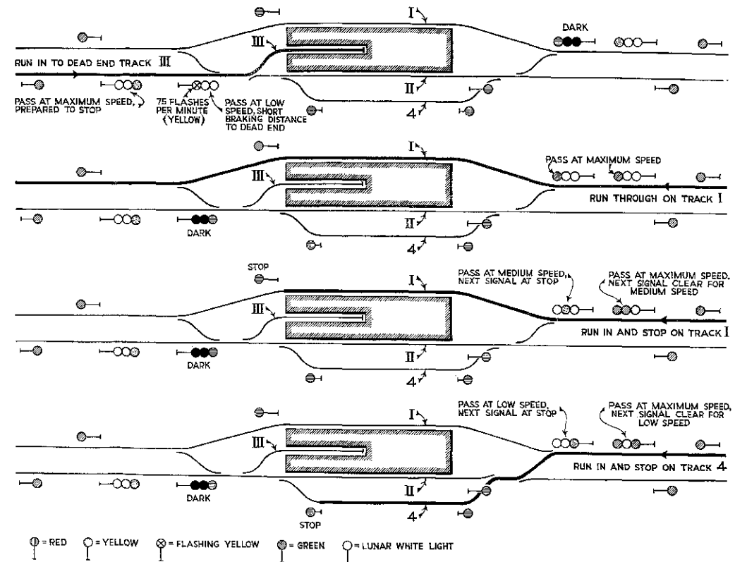
Fig. 5(b) Diagram showing application to typical station layout of new Netherlands speed signalling indications
