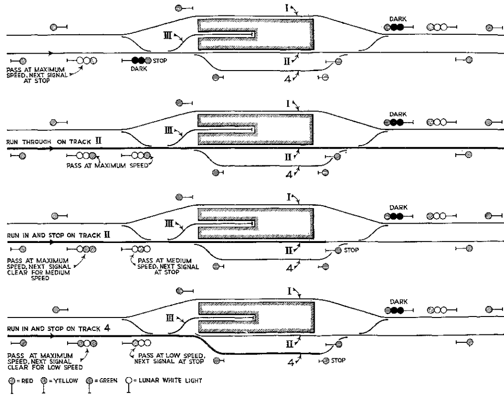
Fig. 5(a) Diagram showing application to typical station layout of new Netherlands speed signalling indications
