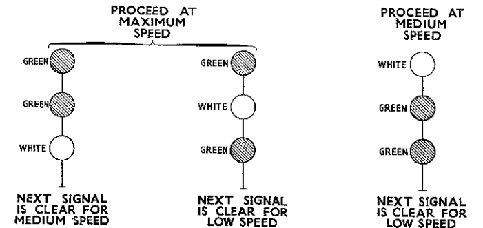
Fig. 4 Proceed indications when signal ahead imposes a lower speed
