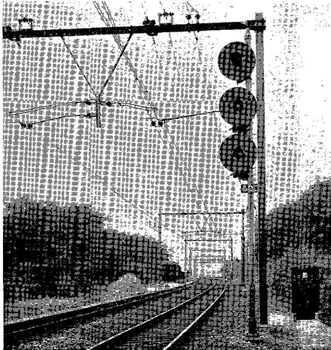
Three-speed multiple-aspect home signal at approach to a station, Netherlands Railways; trains run right-handed
