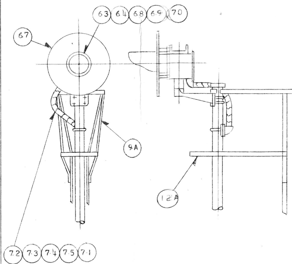
H-5 UNITS MOUNTED FRONT OF MAST AT TOP, MIDDLE OR BOTTOM LOCATION (TOP LOCATION SHOWN)
