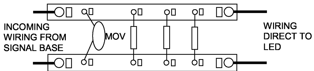
Acceptable concept arrangement showing multiple resistors Connected across signal head terminals.
