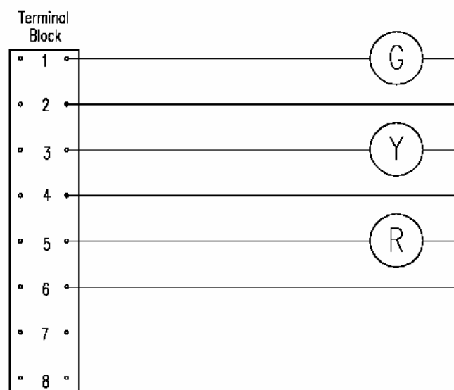
Figure 13-6 Main Line Lampcase – LED Lamps Internal Circuit Double Head Signals - Lower Lampcase 120 Volt 50hz or 12 Volt DC signal lighting supply.
