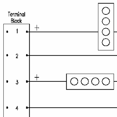
Figure 13-4 Mainline Signal Repeater – LED Lamps 120 Volt 50hz or 12Volt DC signal lighting supply.
